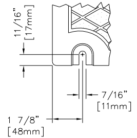
BOLT SLOT DETAIL
