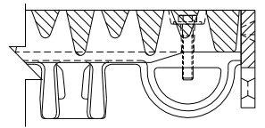
FRAME & COVER SHOWING DEBRIS CHUTE SCALE 1:4
