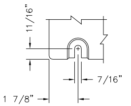
BOLT SLOT DETAIL SCALE 1:4
