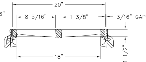
R-4999-FX TYPE "P" GRATE WITH TYPE "B" FRAME TYPICAL SECTION
