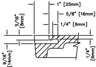
CONCEALED PICKHOLE DETAIL
