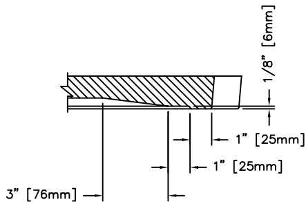
OPEN PICKHOLE DETAIL SCALE 1:4
