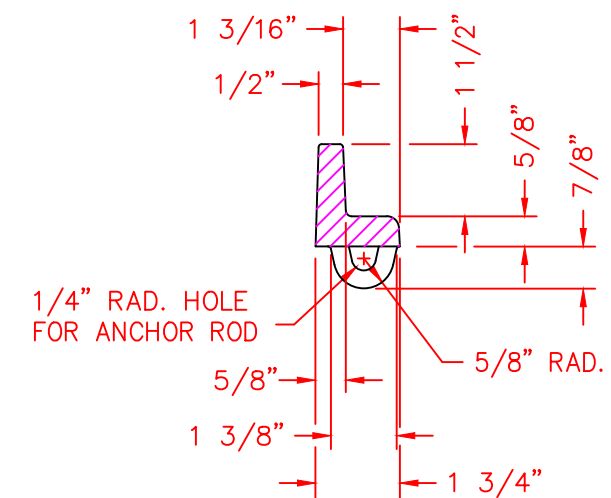
TYPICAL FRAME SECTION SCALE 1:4
