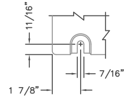
BOLT SLOT DETAIL QUARTER SCALE
