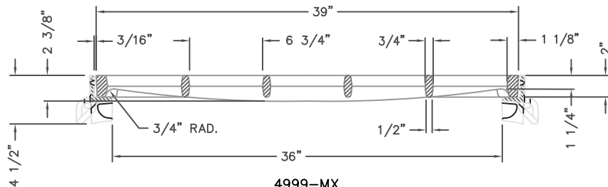
4999-MX SECTION VIEW TYPE "A" GRATE TYPE "B" FRAME
