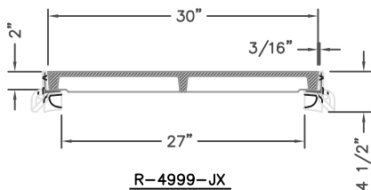
R-4999-JX TYPE "D" LID w/ TYPE "B" FRAME TYPICAL SECTION THROUGH TRENCH
