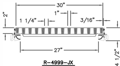
R-4999-JX TYPE "C" GRATE w/ TYPE "B" FRAME TYPICAL SECTION THROUGH TRENCH
