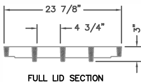
FULL LID SECTION
