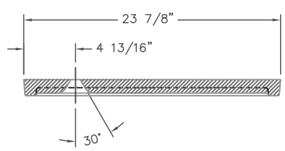
FULL LID SECTION
