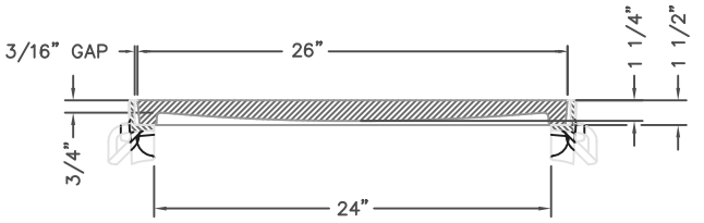
R-4999-HX D TYPE "D" LID w/ TYPE "B" FRAME TYPICAL SECTION THROUGH TRENCH
