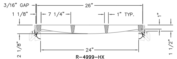
R-4999-HX TYP. SECTION TYPE "A" GRATE AND TYPE 'B' FRAME
