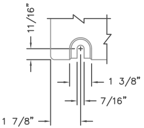
BOLT SLOT DETAIL SCALE 1:4
