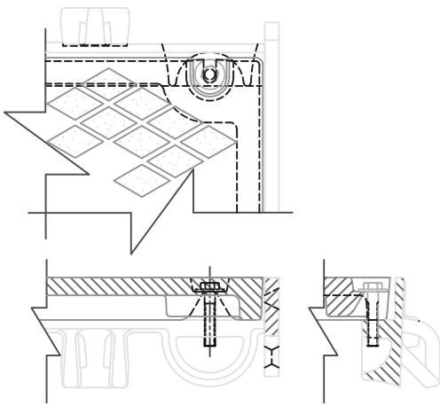
FRAME & LID SHOWING DEBRIS CHUTE
