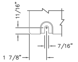
BOLT SLOT DETAIL
