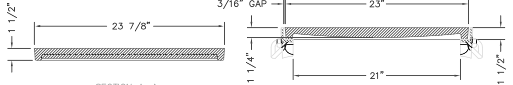
R-4999-GX D TYPE "D" LID WITH TYPE "B" FRAME TYPICAL SECTION
