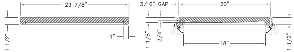
R-4999-FX TYPE "D" COVER WITH TYPE "B" FRAME TYPICAL SECTION
