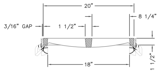
R-4999-FX TYPE "A" GRATE WITH TYPE "B" FRAME TYPICAL SECTION
