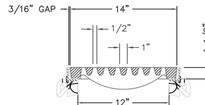
R-4999-DX TYPE "Q" GRATE w/ TYPE "B" FRAME TYPICAL SECTION
