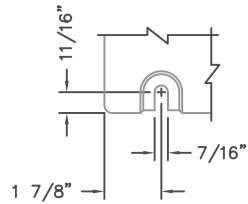
BOLT SLOT DETAIL SCALE 1:4
