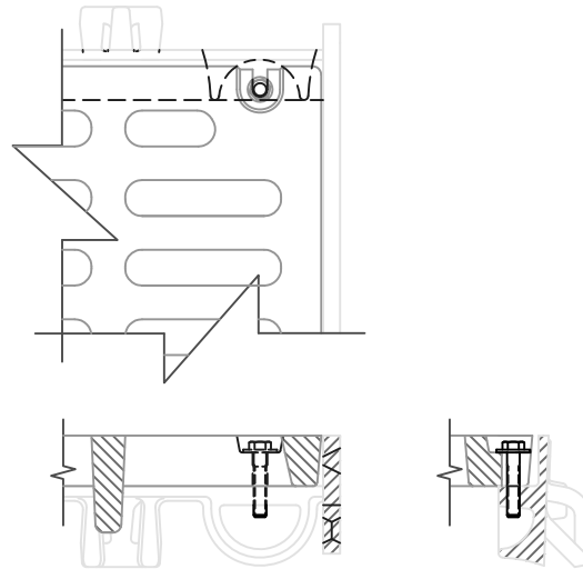
FRAME & GRATE SHOWING DEBRIS CHUTE SCALE 1:4
