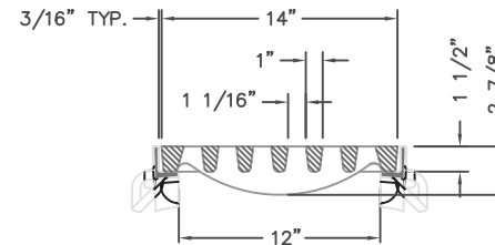
R-4999-DX TYPE "C" GRATE w/ TYPE "B" FRAME TYPICAL SECTION
