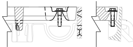
FRAME & GRATE SHOWING DEBRIS CHUTE SCALE 1:4
