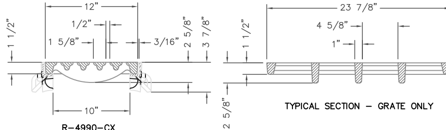
R-4990-CX TYPE "Q" GRATE w/ TYPE "B" FRAME BOLTED TYPICAL SECTION THRU TRENCH
