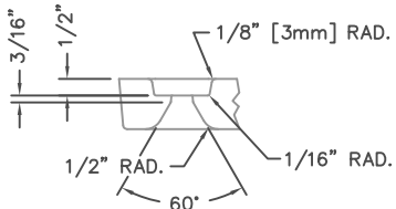
BOLT SLOT DETAIL SCALE 1:4
