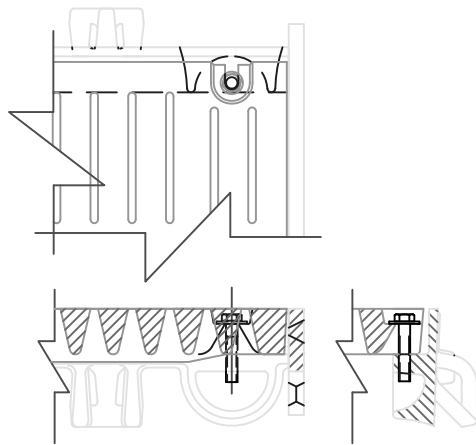
FRAME & GRATE SHOWING DEBRIS CHUTE SCALE 1:4
