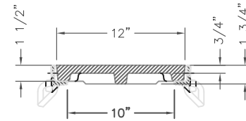
R-4999-CX TYPE "D" LID WITH TYPE "B" FRAME TYPICAL SECTION
