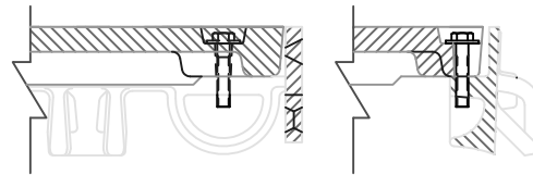
FRAME & LID SHOWING DEBRIS CHUTE SCALE 1:4
