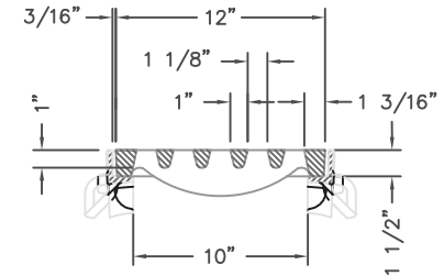
R-4999-CX TYPE "C" GRATE WITH TYPE "B" FRAME TYPICAL SECTION
