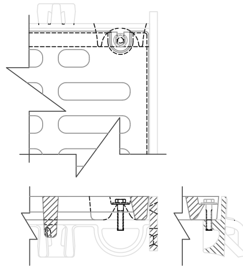
FRAME & GRATE SHOWING DEBRIS CHUTE
