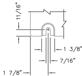
BOLT SLOT DETAIL SCALE 1:4
