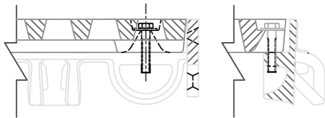
FRAME & GRATE SHOWING DEBRIS CHUTE SCALE 1:4
