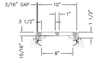
R-4999-BX TYPE "A" GRATE WITH TYPE "B" FRAME TYPICAL SECTION
