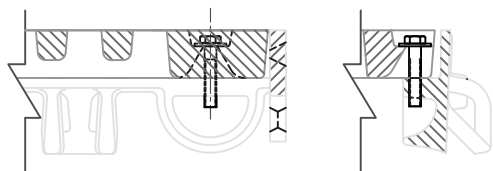
FRAME & GRATE SHOWING DEBRIS CHUTE SCALE 1:4
