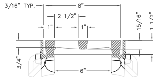
R-4999-AX TYPICAL SECTION TYPE "A" GRATE w/ TYPE "B" FRAME SCALE 1:4
