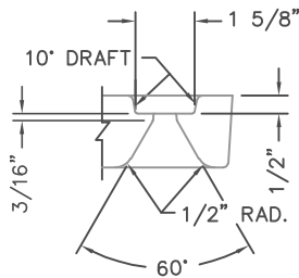
BOLT SLOT DETAIL QUARTER SCALE
