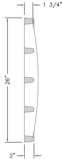
SECTION B-B
