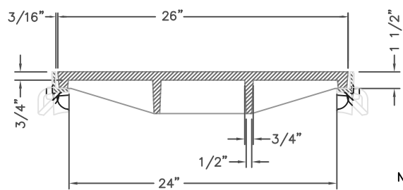
R-4999-HX TYPE "E" LID w/ TYPE "B" FRAME TYPICAL SECTION THROUGH TRENCH
