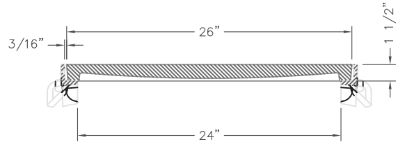
R-4990-HX TYPE "D" LID & TYPE "B" FRAME TYPICAL SECTION
