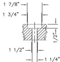
TYPICAL BOLT SLOT DETAIL SCALE 1:4
