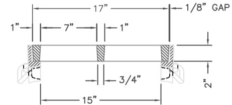
R-4990-EA BOLTED TYPE "A" GRATE AND TYPE "B" FRAME TYPICAL SECTION
