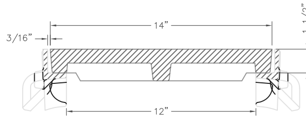
R-4990-DX TYPE "E" LID w/ TYPE "B" FRAME TYPICAL SECTION (SCALE: 1/4"=1")
