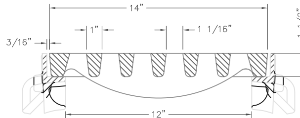
R-4990-DX TYPE "C" GRATE w/ TYPE "B" FRAME TYPICAL SECTION (SCALE: 1/4"=1")
