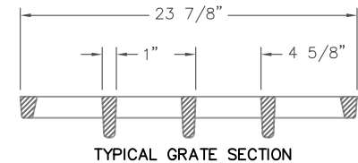
TYPICAL GRATE SECTION
