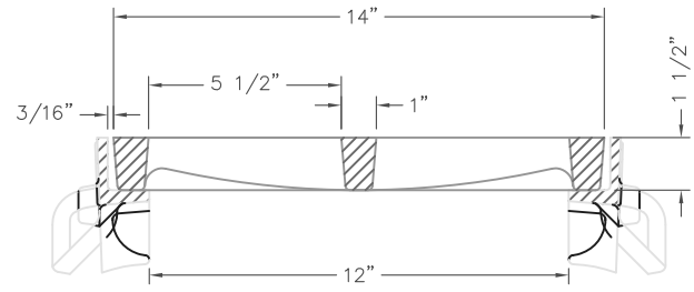
R-4990-DX TYPE "A" GRATE w/ TYPE "B" FRAME TYPICAL SECTION (SCALE: 1/4"=1")
