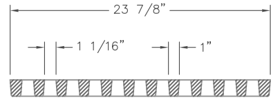
TYPICAL GRATE SECTION
