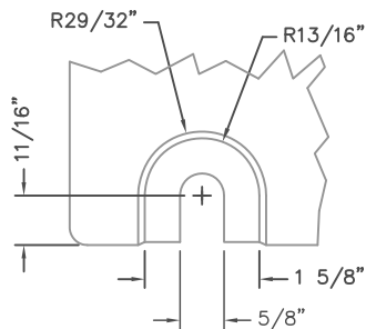
TYPICAL BOLT SLOT DETAIL SCALE 1:2
