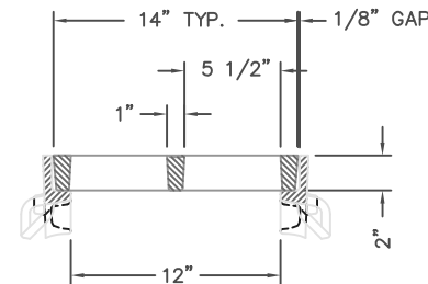
R-4990-DA BOLTED TYPE "A" GRATE AND TYPE "B" FRAME TYPICAL SECTION
