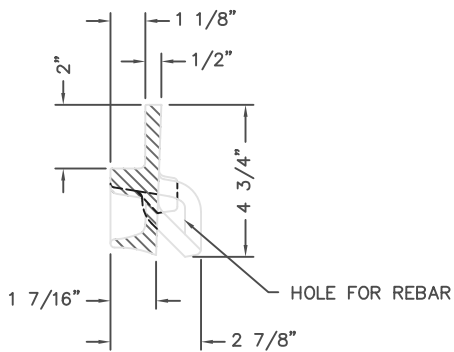
FRAME SECTION VIEW SCALE 1:4
