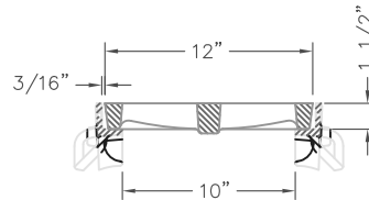
R-4990-CX TYPE "P" GRATE WITH TYPE "B" FRAME TYPICAL SECTION
