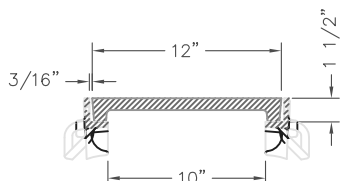
R-4999-CX TYPE "E" LID WITH TYPE "B" FRAME TYPICAL SECTION
