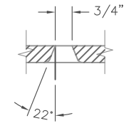
VENT HOLE DETAIL SCALE 1:4
