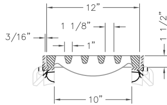
R-4999-CX TYPE "C" GRATE WITH TYPE "B" FRAME TYPICAL SECTION
