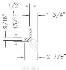
SECTION VIEWS
