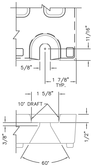
BOLT SLOT DETAIL SCALE 1:2
