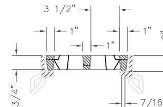
R-4990-BA AIRPORT TRENCH TYPE "A" GRATE w/ TYPE "B" FRAME TYPICAL SECTION
