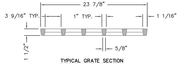
TYPICAL GRATE SECTION
