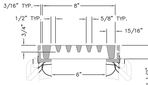
R-4999-AX TYPICAL SECTION TYPE "Q" GRATE w/ TYPE "B" FRAME (SCALE: 1/4"=1")
