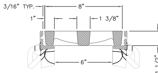
R-4990-AX TYPICAL SECTION TYPE "P" GRATE w/ TYPE "B" FRAME (SCALE: 1/4"=1")
