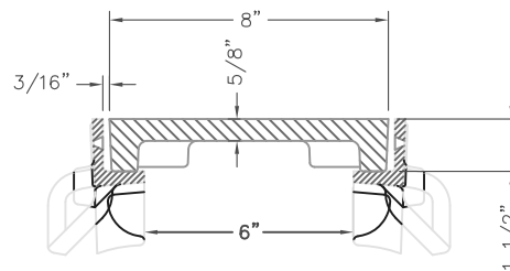
R-4990-AX TYPICAL SECTION TYPE "P" GRATE w/ TYPE "B" FRAME (SCALE: 1/4"=1")
