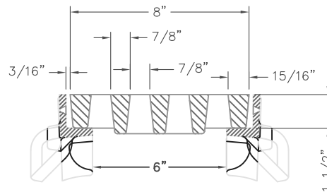
R-4990-AX TYPICAL SECTION TYPE "P" GRATE w/ TYPE "B" FRAME (SCALE: 1/4"=1")
