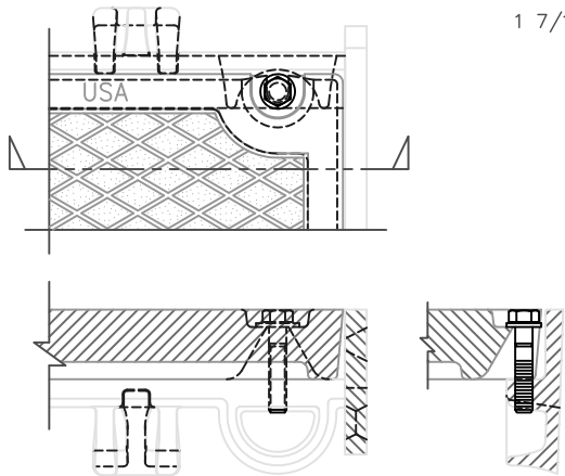
FRAME AND COVER SHOWING DEBRIS CHUTE SCALE 1:4
