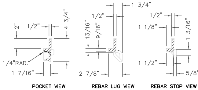
SIDE FRAME SECTION VIEWS
