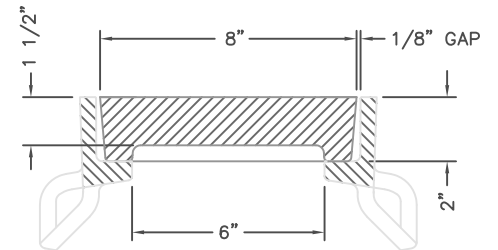
R-4990-AA BOLTED TYPE "D" LID AND TYPE "B" FRAME TYPICAL SECTION SCALE 1:4
