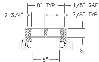
R-4990-AA BOLTED TYPE "A" GRATE AND TYPE "B" FRAME TYPICAL SECTION
