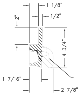
FRAME SECTION VIEW SCALE 1:4
