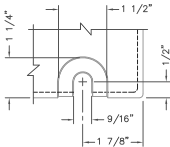
TYPICAL BOLT SLOT DETAIL SCALE 1:2
