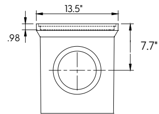
CATCH BASIN OPTIONAL EXTENSION
