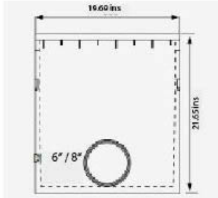
Catch Basin includes galvanized dirt catcher
