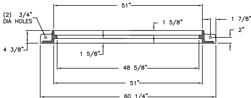
GRATE SECTION
