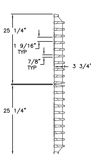
GRATE SECTION
