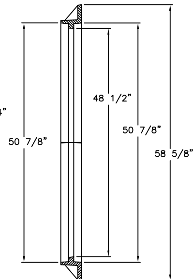
FRAME SECTION
