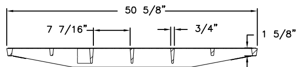
GRATE SECTION
