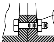
TWO PIECE FRAME BOLTDOWN DETAIL
