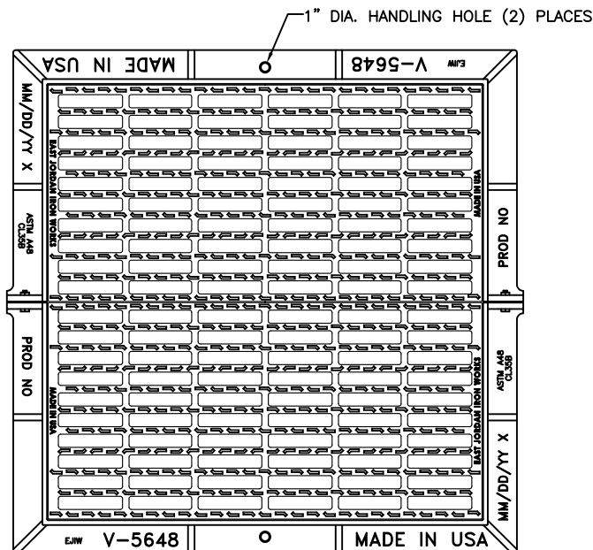
FRAME AND GRATE TOP VIEW
