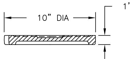
COVER SECTION
