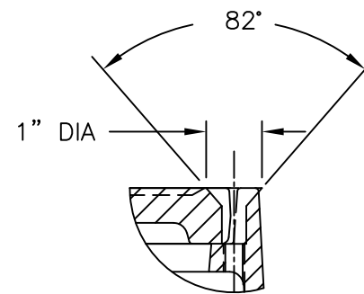
CRACK DRILL DETAIL
