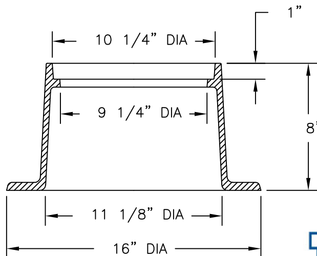
FRAME SECTION
