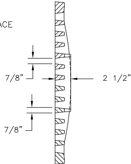
GRATE SECTION
