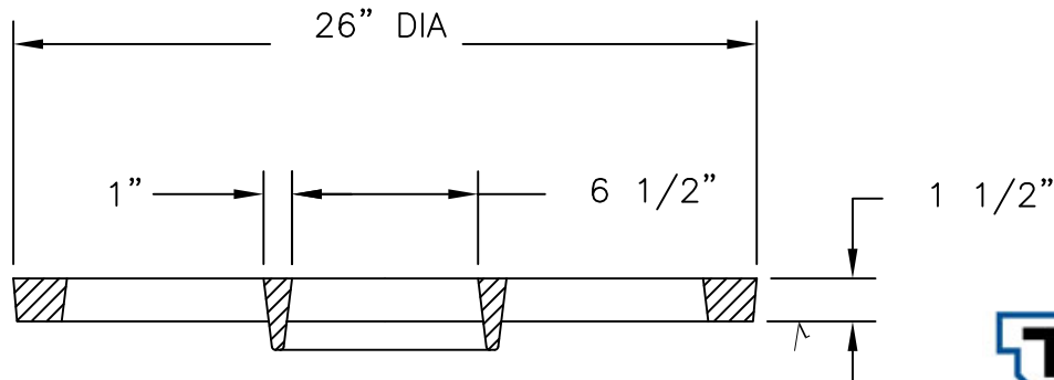
GRATE SECTION
