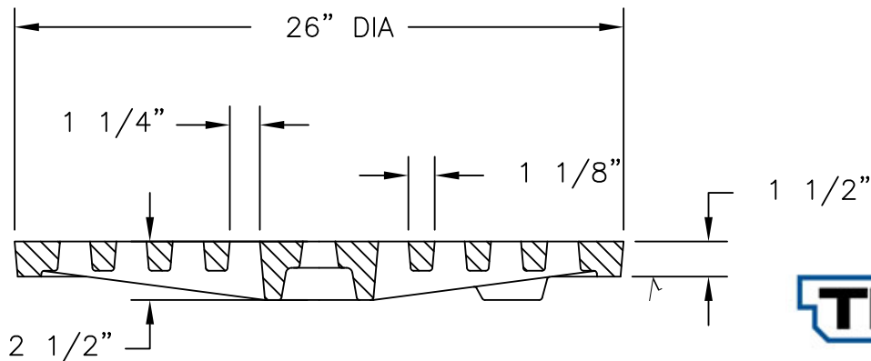
GRATE SECTION
