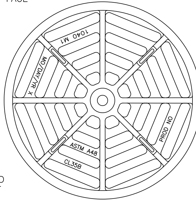
BOTTOM VIEW OF GRATE
