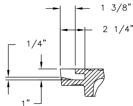
PICKHOLE DETAIL
